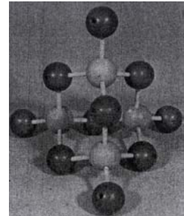
Phosphorpentoxid ( P_4O_{10} )
